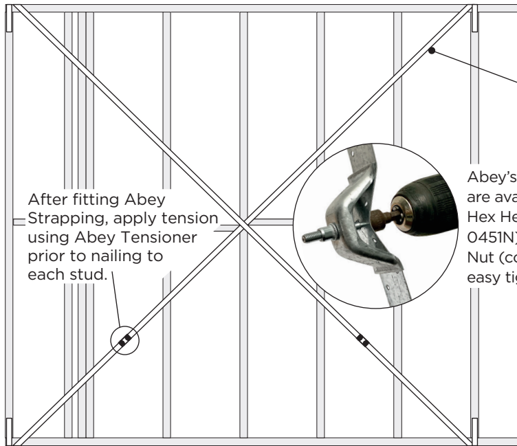
Single section of Abey Strapping 30mm x 0.8mm
